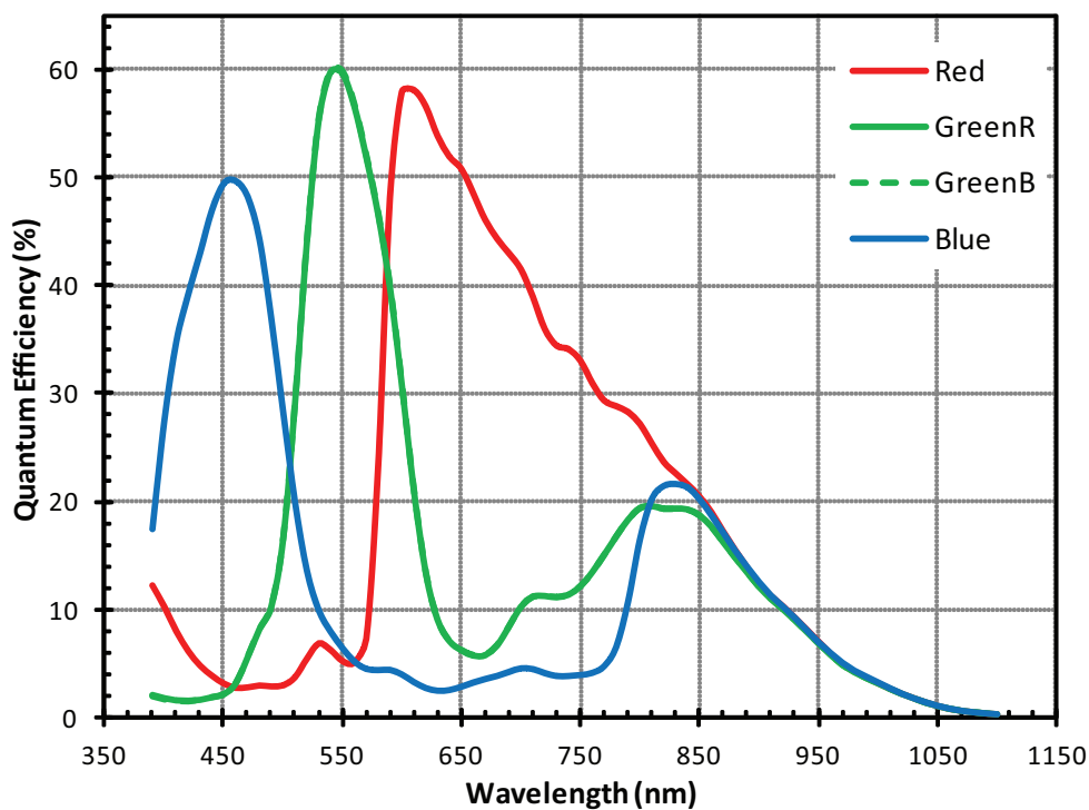
Figure 50: Quantum Efficiency
