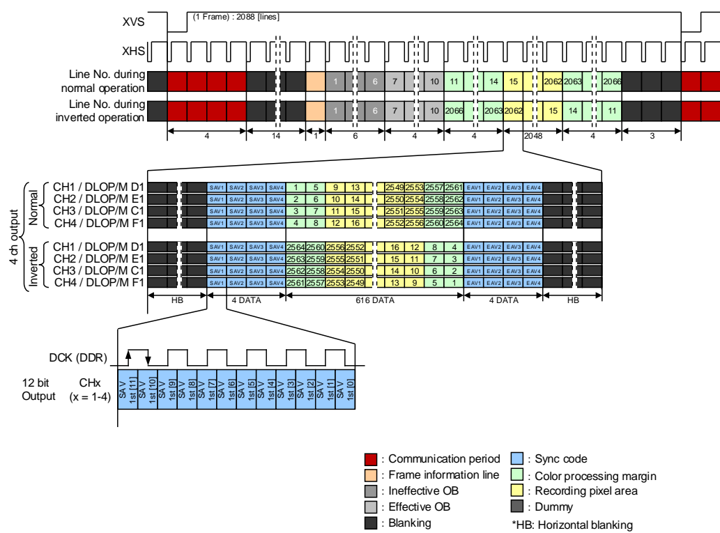
Drive Timing Chart for Serial Output in All-pixel Scan Mode
