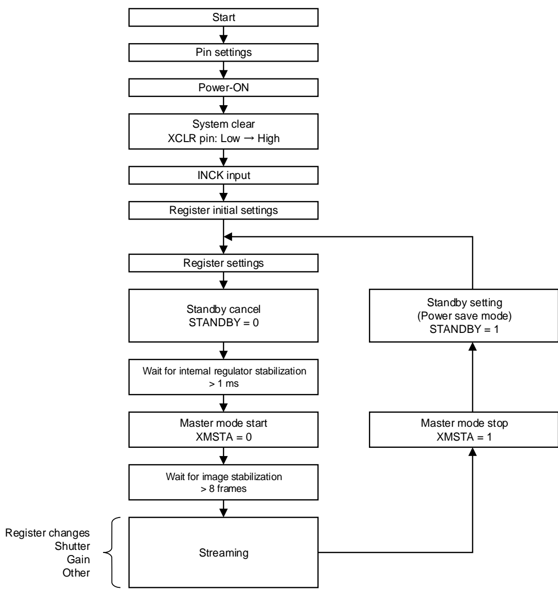
Sensor Setting Flow (Sensor Master Mode)
