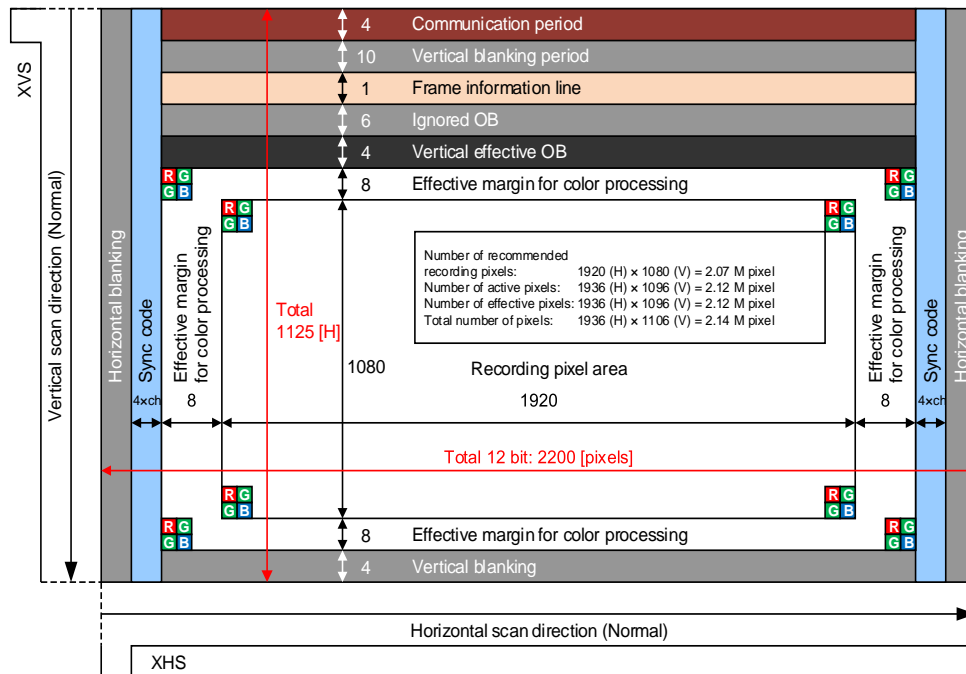
Pixel Array Image Drawing in 1080p-Full HD Mode
