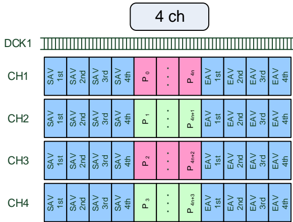
Output Format of Low voltage LVDS Serial 4 ch
