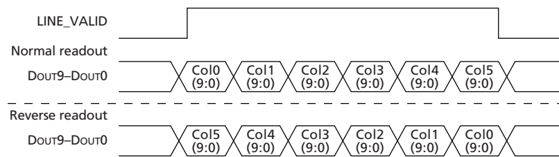
Figure 11: Readout of Six Columns in Normal and Column Mirror Output Mode
