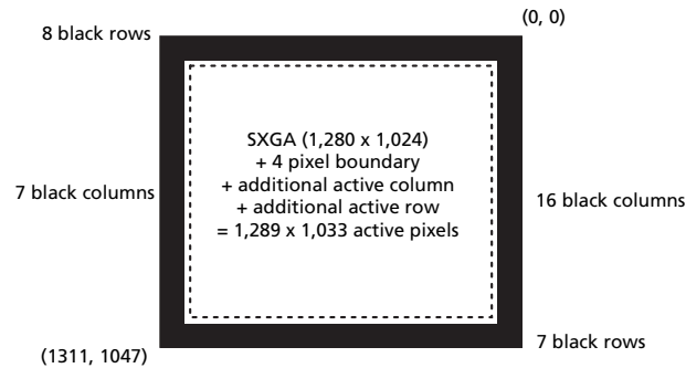
Figure 3: Pixel Array Description
