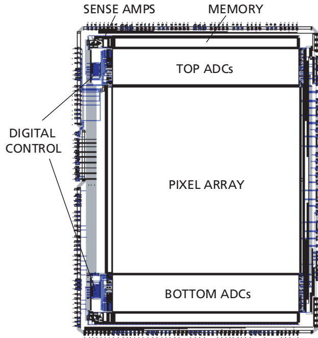
Figure 2: Sensor Architecture (not to scale)
