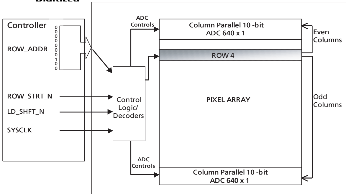
Figure 5: Example 1 - Row 4 of the MT9M413 Being Digitized
